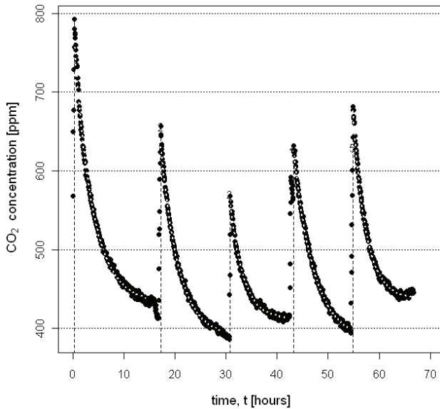
Fig. 4. Decay curves of CO 2 (black glyphs) in a bedroom equipped with double box window and located in a building built in 1908, estimated with nonlinear regression (white curves).
