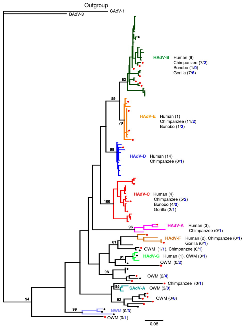
Figure 1. DPOL sequence-based phylogenetic analysis. Partial DPOL gene sequences from the novel AdVs and from published NHP AdVs and human AdVs were aligned and subjected to phylogenetic analysis. The tree was reconstructed using maximum likelihood with the HKY85 model of substitutions, as described in Materials and Methods. AdVs from wild and captive NHPs discovered in this study are marked with red and black dots, respectively. All other NHP AdVs were reported previously and originated from captive animals. The branches of all AdVs that could tentatively be allocated to one of the species Human adenovirus A to G or to the species Simian adenovirus A are colored separately. Branches left without extra coloring belong to AdVs for which allocation to an AdV species was not possible. Bootstrap values are depicted at the nodes of the tree; nonsignificant values or those close to branch tips were omitted. AdV species and host compositions are indicated on the right. Numbers of AdVs found in each host species are given in parentheses: numbers of published AdVs are given before the slash, in black, and numbers of novel AdVs from this study are given behind the slash, in blue.
