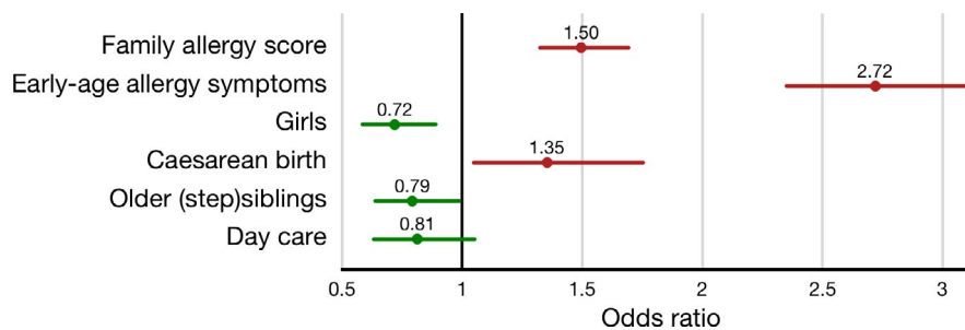
FIGURE 3 Odds ratios and 95% confidence intervals for protective factors (green) and risk factors (red) of allergic multimorbidity at school age [of a model selected according to AICc]. Family-allergy-score is standardized to have SD = 1. Early-age-symptoms is in the range 1–3 and counts the number of allergic symptoms (of allergic rhinitis, eczema, asthma) observed before age 2. All the remaining variables are dichotomous. The OR for family-allergy-score shows the multiplicative effect for each standard deviation, and somewhat similarly, the OR for early-age symptoms shows the multiplicative effect of each such symptom that is present. The factors shown are the ones present in a multivariate logistic model that maximizes the AICc model selection criterion
