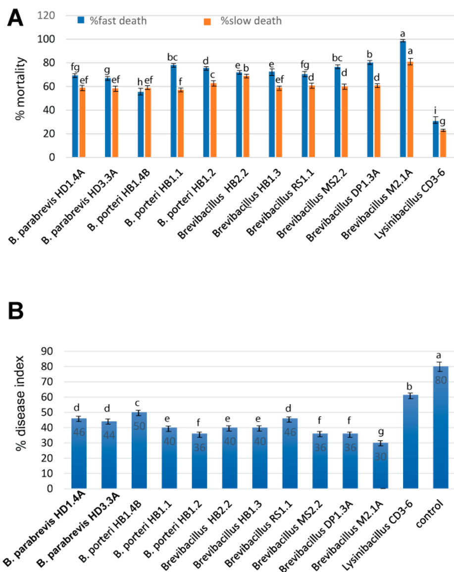
Figure 6. Nematicidal activity of Brevibacillus strains and Lysinibacillus CD3-6. (A): Bioassay with Caenorhabditis elegans . Slow killing activity was determined on NGM plates, and fast killing activity in liquid medium. (B): Tomato plants were infested with the root-knot nematode Meloidogyne sp. and the root-knot-forming rate in the presence and absence of the bacterial strains was estimated after 10 weeks growth of the tomato plants under controlled conditions in a greenhouse. All experiments were carried out with three independent repetitions and a completely randomized design. Different letters at each treatment indicate the significance between inoculated and uninoculated conditions at the p \leq 0.05 level after the t -test.
