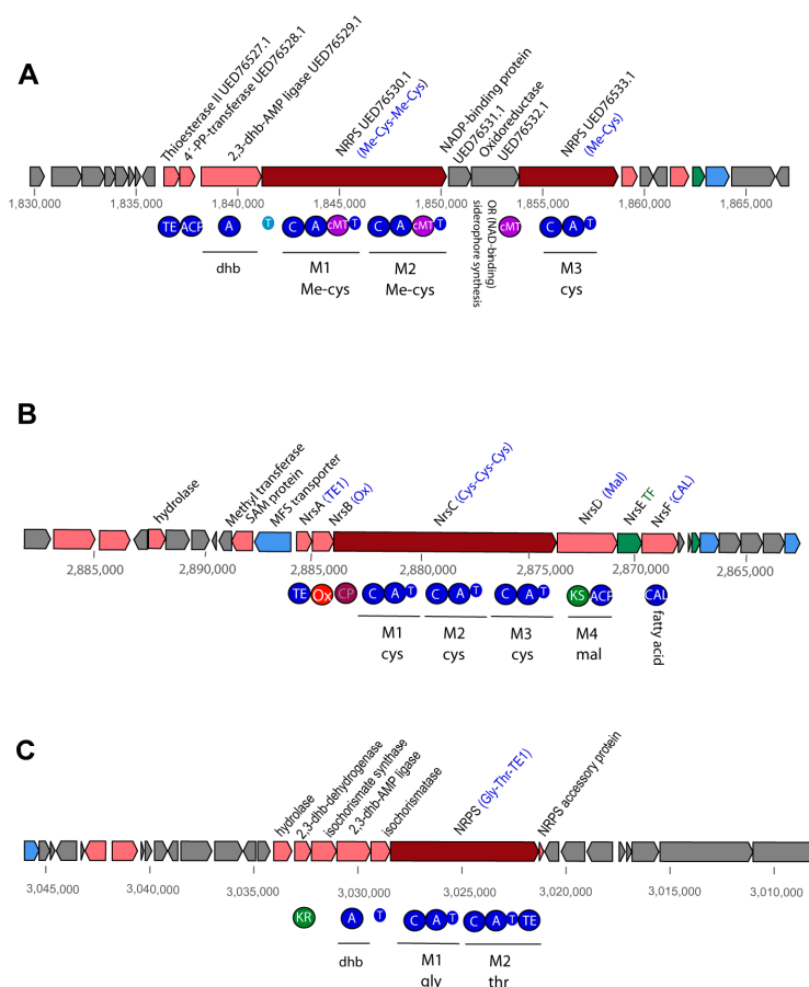
Figure 10. The uncharacterized NRPS gene cluster in Brevibacillus sp. DP1.3A (A) compared with the Bacillothiazol synthesizing nrs gene cluster (B) and the siderophore bacillibactin dhb gene cluster in Bacillus velezensis FZB42 (C). NRPS/PKS domains are indicated by filled circles. A: adenylation, ACS: 4'-phosphopantetheinyl transferase, C: condensation, CAL: co-enzyme A ligase, cMT: carbon methyltransferase, KR: ketoreductase, KS: ketosynthase, T: thiolase, TE: thioesterase.
