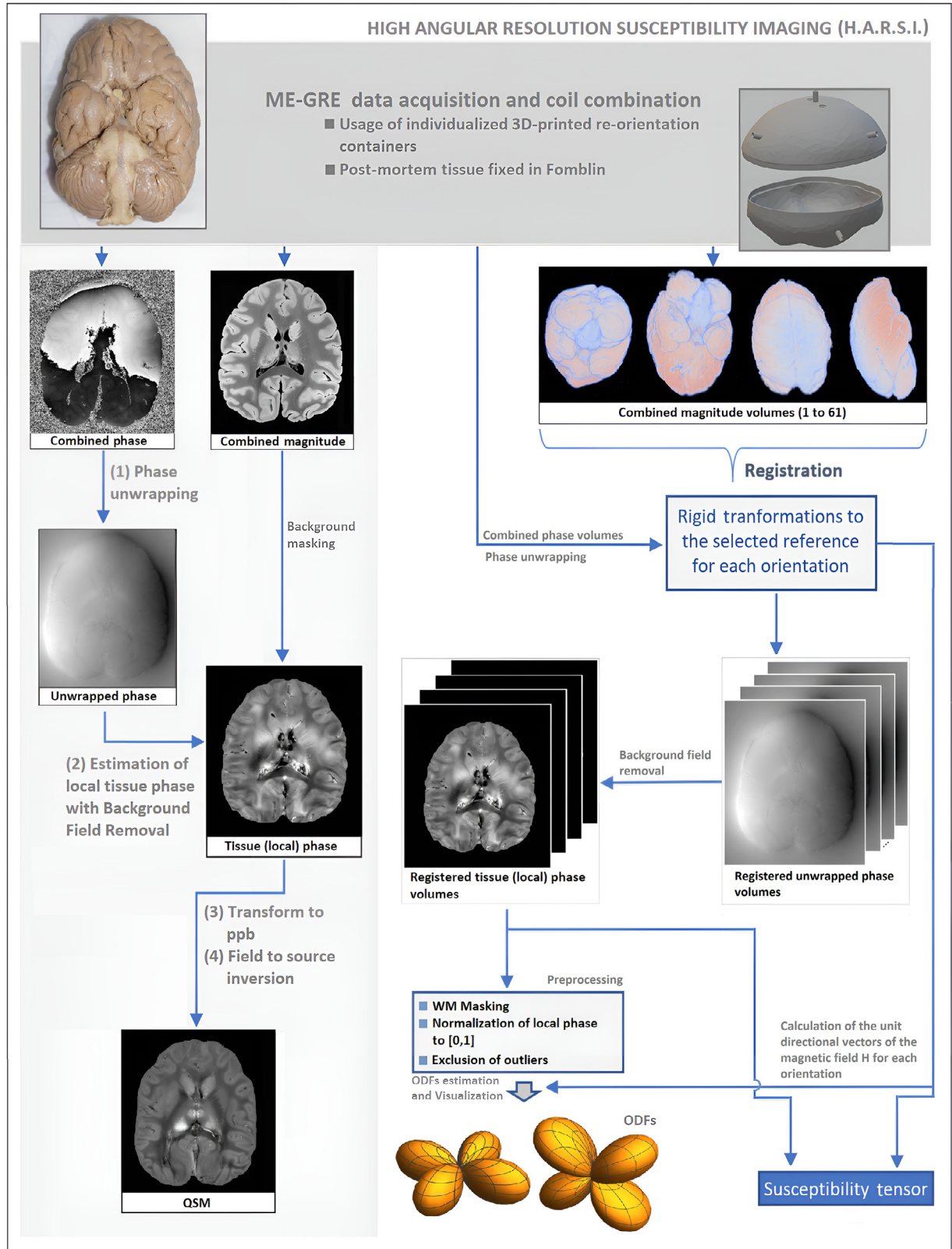
Fig. 2. Simplified schematics of the pipelines employed for QSM as well as STI and ODF derivation from high-angular GRE phase data. The complex-valued GRE data from each of the 32 coil channels are saved individually and combined using SVD-ESPIRiT. (Left) QSM pipeline starting with Laplacian phase unwrapping on the combined raw phase and local \delta B_0 estimation with background-field removal using V-SHARP and, finally, field-to-source inversion, to obtain relative \chi values employing iLSQR. (Right) STI and HARSI pipeline with registration of the multi-orientation phase volumes to a reference employing transformations derived from registrations of the corresponding magnitude volumes. Phase unwrapping and background-field removal is performed individually for each orientation. iLSQR is also employed for susceptibility-tensor reconstruction. For ODF estimation, further pre-processing (masking, normalization, outlier removal) is required.
