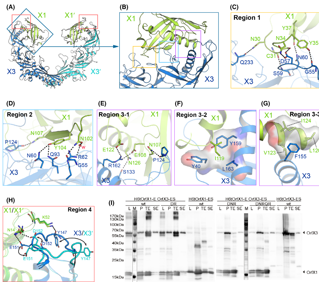
Fig. 2. Interactions between OrfX1 and OrfX3. (A) Overall structure of the OrfX1-OrfX3 complex. (B) Close-up view of the OrfX1-OrfX3 heterodimer interface with the three major interacting areas highlighted in boxes. (C-G) Stick representations of key interacting residues at the OrfX1-OrfX3 interface. Hydrogen bonds are shown as dashed lines and hydrophobic interactions are shown as surface models. (H) The E144-D153 loop in the two OrfX3 molecules in the context of the OrfX1-OrfX3 complex, coloured blue and cyan, displays different conformations. (I) Co-expression analysis of the WT H6tOrfX1-ES, WT H6tOrfX3-ES, H6tOrfX1-OrfX3-ES WT complex and the respective OrfX3 mutants D152R/R162A (DR), D57A/N60A/R62A (DNR), and D57A/N60A/R62A/Q93A/R162A (DNRQR) ( n = 2-4 ). L, clear lysate; P, cell pellet after lysis; TE, eluate from Co 2+ -Talon matrix; SE, eluate from StrepTactin matrix. Samples were analysed by immunoblot using anti-OrfX1-3 specific polyclonal rabbit IgG KOrf154. The corresponding SDS/PAGE and Coomassie staining result is shown in Fig. S2.
