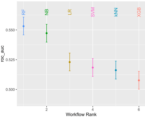
Fig. 2. Comparison of the machine learning algorithms. Note. Credible intervals derived from the Bayesian random intercept model posterior distributions. roc_auc = the area under the receiver operating characteristic curve; RF = Random Forest; NB = Naive Bayes; LR = Logistic Regression; SVM = Radial basis function support vector machines via kernlab; kNN = k-Nearest-Neighbor; XGB = XGBoost.
