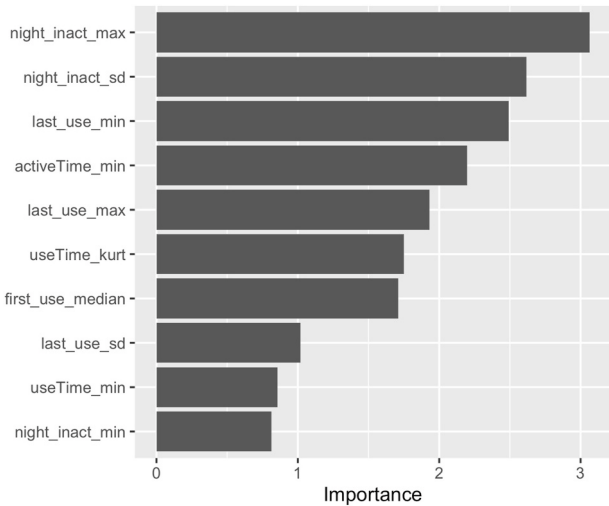
Fig. 3. Variable importance plot Random Forest.
