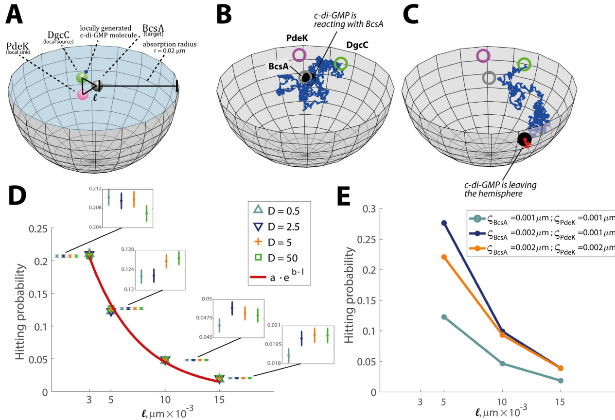
Figure 7. Mathematical modeling of local c-di-GMP signaling by BcsA, DgcC and PdeK interaction. (a) Setup of the modeled system. BcsA, DgcC and PdeK were placed in an equilateral triangle with side length l on the cell membrane. A hemisphere, centered around BcsA, with radius r = 0.02 \mu\text{m} defines an absorption radius; i.e. when c-di-GMP leaves this hemisphere, it is considered to be eliminated by a global sink (i.e. PdeH). (b) Trajectory (blue line) hitting BcsA. The solid black circle indicates the position of c-di-GMP when it enters the reaction radius of BcsA. (c) Trajectory before (blue line) and shortly after (red line) leaving the local hemisphere, after which it is unlikely to hit the local target. The solid black circle indicates the position of c-di-GMP when it leaves the hemisphere. Gray, green and magenta circles represent the reaction radii of BcsA, DgcC and PdeK, respectively. (d) Dependency of the hitting probability on the DgcC–BcsA–PdeK distance l and diffusion coefficient D for a reaction radius \rho = 0.001 \mu\text{m} . The red curve is an exponential function with fitted parameters a and b (see Supplementary Information) that depends on the DgcC–BcsA–PdeK distance l . Error bars represent 95% confidence interval for data presented on the left, calculated with Greenwood's formula. (e) Dependency of the hitting probability on the DgcC–BcsA–PdeK distance l and reaction radius \rho . A minimum distance ( l = 5 \text{ nm} ) was chosen that exceeds all considered reaction radii.
