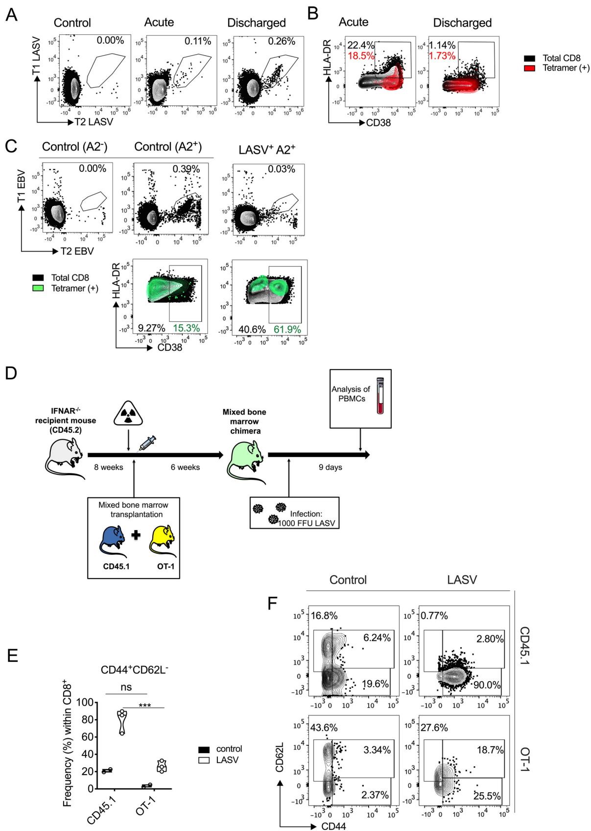
FIG 2 T-cell activation during acute Lassa fever (LF). (A) HLA-A2 tetramers labeled with two fluorophores (T1 and T2, respectively) were utilized to track epitope-specific CD8 T cells during acute LF. The plots show results for pooled (concatenated) samples from LF patients ( n = 3 )
