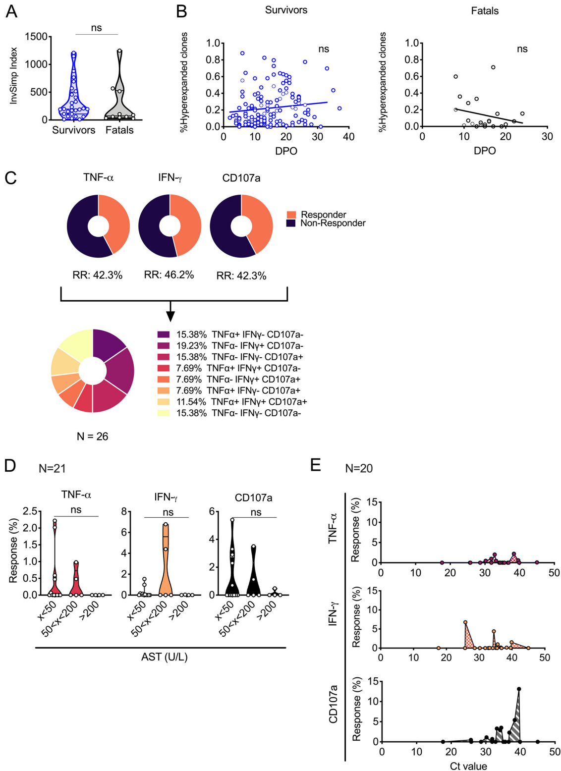
FIG 3 Clonal repertoires and effector T-cell responses in Lassa fever (LF) patients. (A) Cross-sectional T-cell repertoire diversity in LF survivors ( n = 28 ) and fatal cases ( n = 10 ) was analyzed by TCR sequencing and is represented as the inverse of Simpson's index (InvSimp). Violin plots depict individual samples, sample distributions, median values, and quartiles. Statistical significance was determined using the Mann-Whitney test, and significance levels are presented as follows: ns, P > 0.05 (not significant); *, P \leq 0.05 ; **, P \leq 0.01 ; ***, P \leq 0.001 ; ****, P \leq 0.0001 . (B) Longitudinal evaluation of hyperexpanded clones (see clonal space definitions in Materials and Methods) in n = 120 samples collected from survivors and n = 22 samples collected from nonsurviving patients. Individual samples and trend lines are depicted. ns, not significant (Spearman's correlation analysis); DPO, days postonset. (C) Pie chart depicting the percentages of patient samples ( n = 26 ) that showed effector response capacity as indicated by production of cytokines (Continued on next page)
