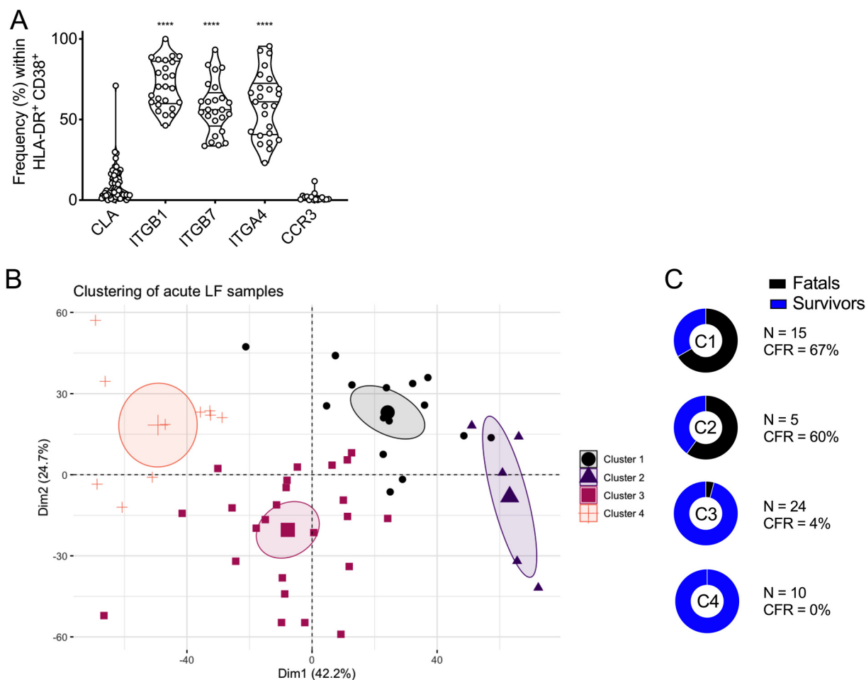
FIG 4 T-cell homing in human LF. (A) Freshly isolated patient PBMCs were analyzed by flow cytometry, and activated (CD38 + HLA-DR + ) CD8 T cells from LF patients were analyzed for expression of the T-cell homing factors ITGB7, ITGA4, ITGB1 ( n = 25 ), CCR3 ( n = 16 ), and CLA ( n = 61 ). Violin plots depict individual samples, sample distributions, median values, and quartiles. Statistical significance was determined using the Kruskal-Wallis test followed by Dunn's posttest, and significance levels are presented as follows: ns, P > 0.05 (not significant); *, P \leq 0.05 ; **, P \leq 0.01 ; ***, P \leq 0.001 ; ****, P \leq 0.0001 . (B) Principal-component analysis (PCA) of T-cell homing markers in the activated compartment (CD38 + HLA-DR + ) of CD4 and CD8 T cells in cryopreserved patient samples ( n = 54 ). Clustering of samples was based on hierarchical analysis to identify main subsets. (C) CFR for each cluster was calculated based on outcome of disease of the corresponding patient linked to each sample. Dim, dimension; C, cluster; CFR, case fatality ratio.
