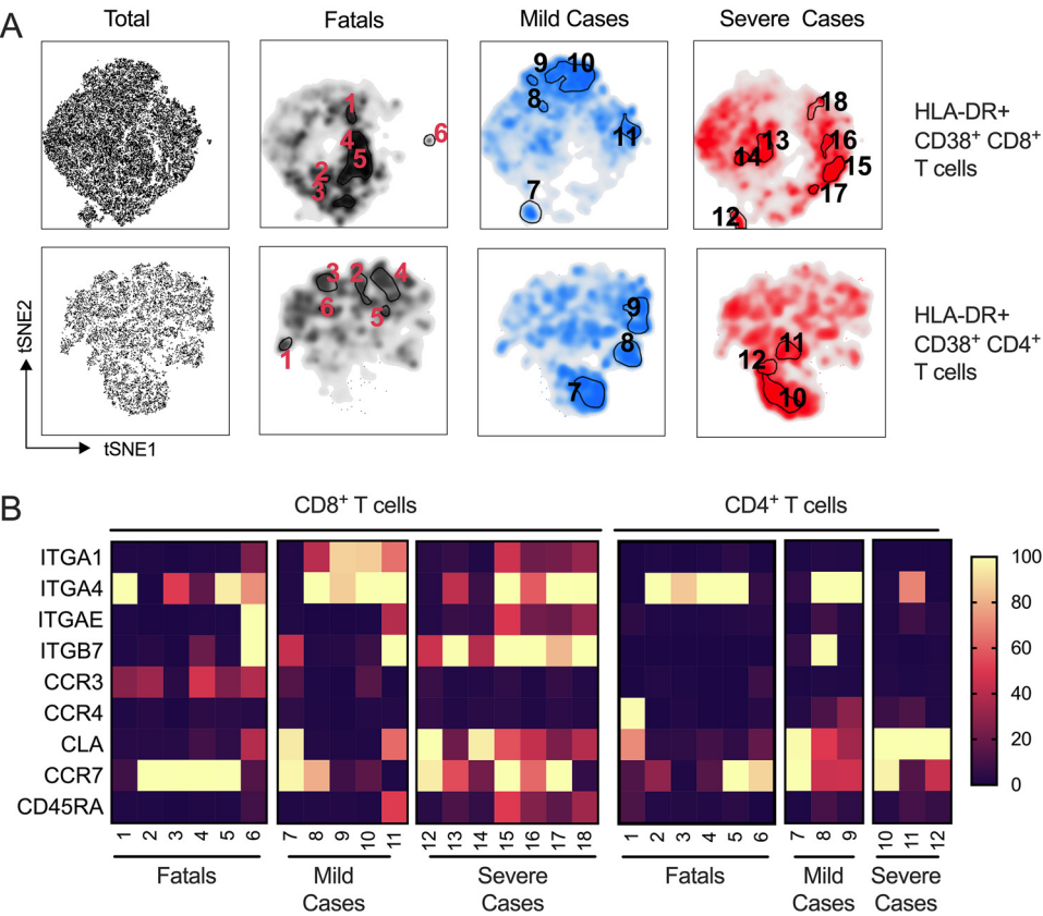
FIG 5 T-cell populations in LF patients. (A) Activated (CD38 + HLA-DR + ) CD8 + and CD4 + T cells were concatenated across all patient samples ( n = 54). t -Distributed stochastic neighboring embedding ( t -SNE) was calculated on the expression of homing markers CLA, CCR3, CCR4, CCR7, ITGA4, ITGA1, ITGAE, and ITGB7 and expression of CD45RA. Outcome-based population analysis was performed by automated density-based gating. Numbers indicate T-cell subsets identified in the t -SNE analysis. (B) For each identified population, the percentage (%) of contribution from each outcome was verified, and the expression frequency (%) of each marker is shown according to the color key on the right. CCR, chemokine receptor; CLA, cutaneous lymphocyte antigen; ITG, integrin.
