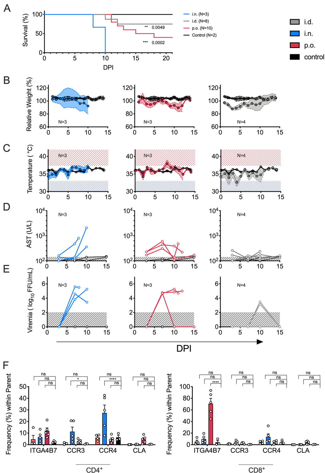
FIG 6 Route-dependent LF severity in mice. (A) IFNAR B6 chimeras were infected with 1,000 FFU of LASV either i.n., p.o., or i.d. Uninfected mice served as the control. Survival is shown in Kaplan-Meier curves. Statistical evaluation was performed via Mantel-Cox test. DPI, days postinfection. (B to E) Longitudinal analysis of morbidity parameters in IFNAR B6 chimeras infected with LASV via different routes, including relative weight loss (B), fluctuations in body temperature (C), levels of serum aspartate (Continued on next page)
