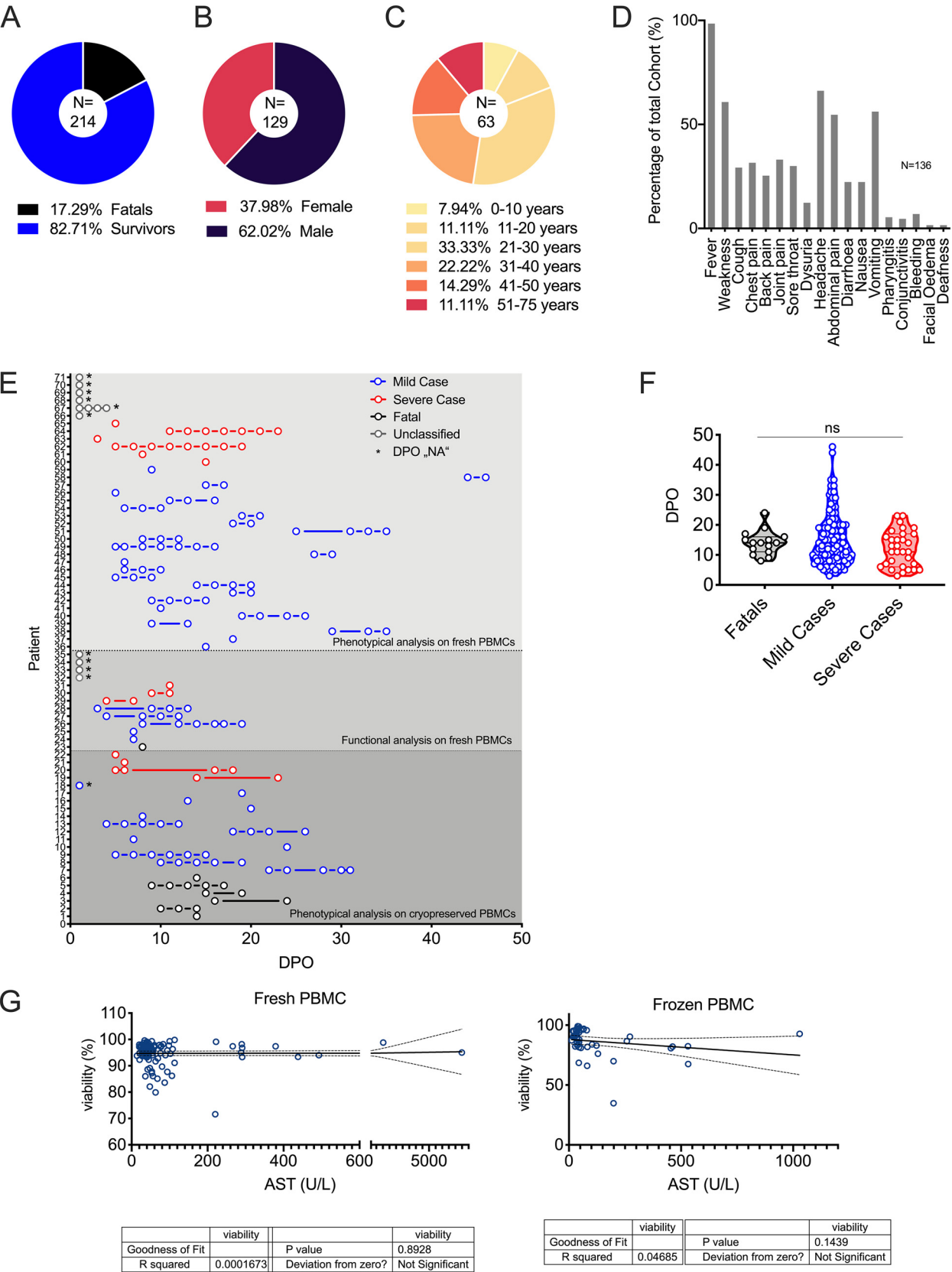
FIG 1 Patient demographics and clinical symptoms. (A to C) Outcome ( n = 214 ) (A), gender ( n = 129 ) (B), and age ( n = 63 ) (C) distributions of patients admitted to the Lassa ward during the study period. Distributions of patients in population are shown as the percentages of the total cohort. Pie chart colors are described in keys below. (D) Symptoms of patients ( n = 136 ) admitted to the Lassa ward. (E) PBMCs in whole-blood samples were analyzed (Continued on next page)
