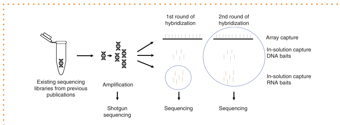
Figure 1. Schematic representation of the workflow. For all samples, the three different enrichment protocols were tested in three independent replicates. Blue circles indicate the libraries that were sequenced at each particular step.
