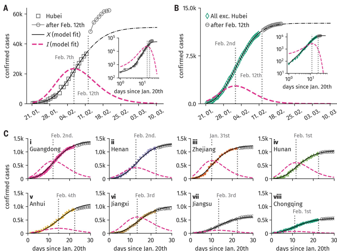
Fig. 2. Case numbers in Hubei compared to model predictions. The quarantined compartment X(t) and the unidentified infectious compartment I(t) are obtained from fits to the model defined by Eqs. 1 to 4 as described in the materials and methods. All fits were performed for case numbers predating 12 February at which the case number definition was temporarily
