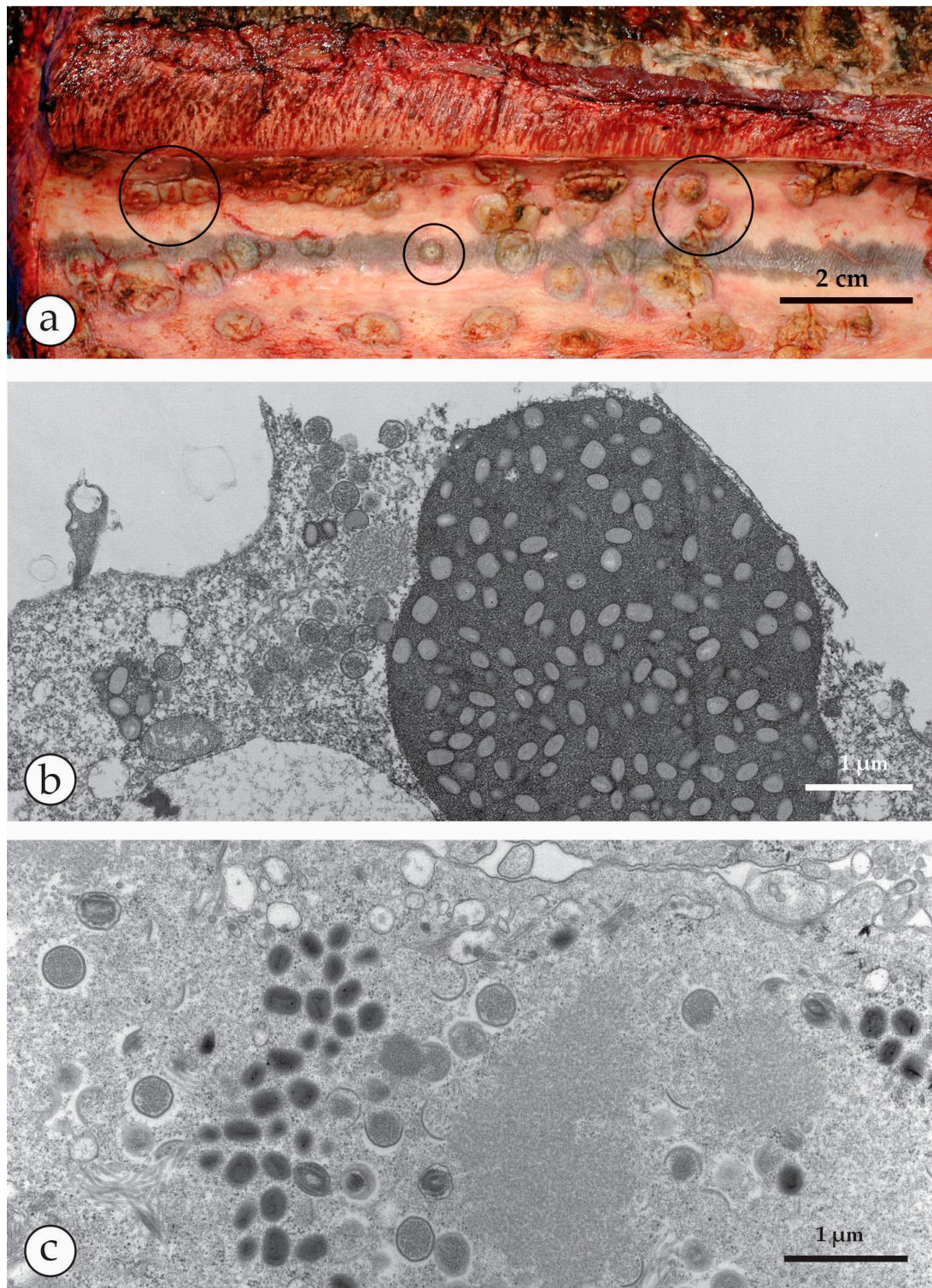
Figure 4. Peculiarities of CPXV infections: wide host range and specific inclusion bodies. (a) Lesions on the inner surface of a trunk of a deceased elephant, sliced longitudinally showing multiple ulcerous lesions on the mucous membranes [34]. Image courtesy Dr. Gudrun Wibbelt, Berlin. (b) After inoculation from the elephant’s ulcers in diagnostic cell cultures, well-circumscribed inclusion bodies developed consisting of a moderately dense matrix that included numerous mature virions. These are type A eosinophilic inclusions as seen in light microscopical histology and called Downie or Marchal bodies. They are typical of CPXV but found with a few other poxvirus genera [35]. (c) OPV are assembled in large cytoplasmic “factories” but these are basophilic (type B inclusions or Guarnieri bodies) in light microcopy and less well circumscribed.
